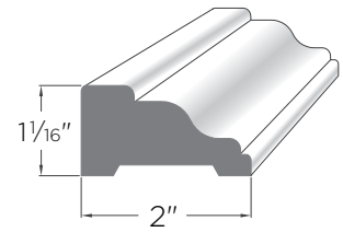
Rake Moulding AZM-287
