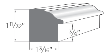
Back Band AZM-6931
