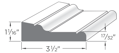
Adams Casing AZM-97
